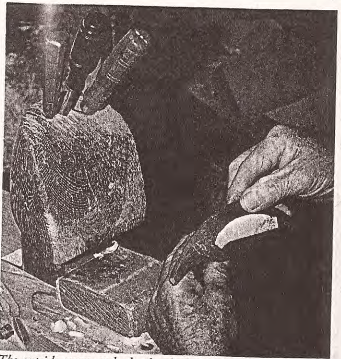
The outside curve and edge bevel of a bucket stave are checked with a gauge called a modell, drawn on facing page.
