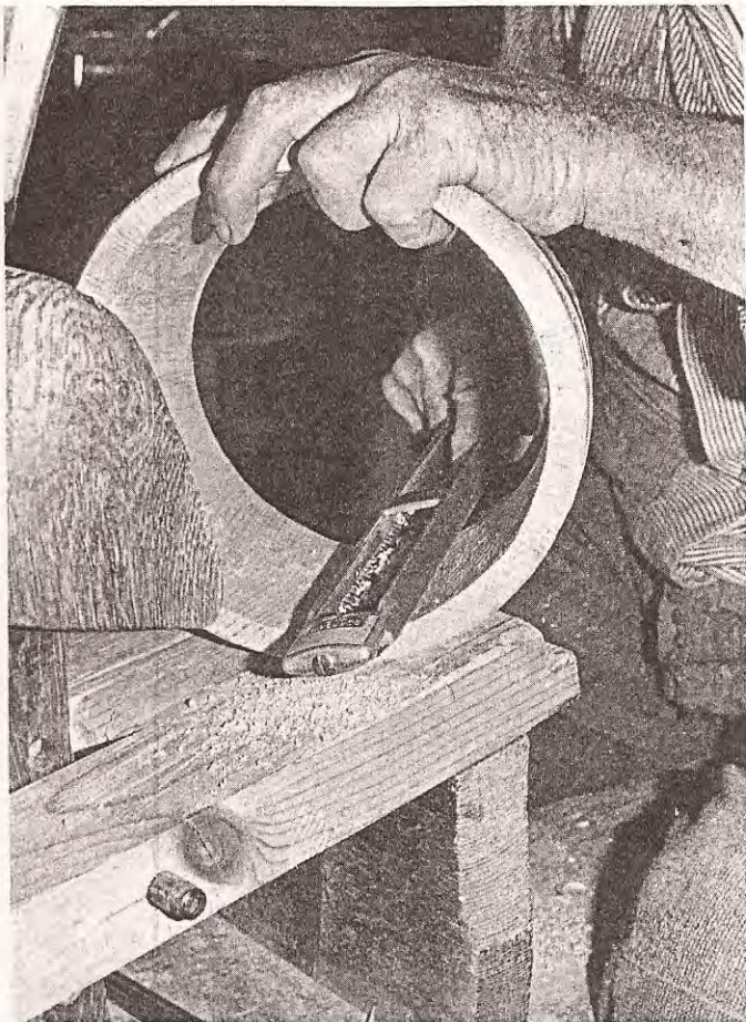
The staves are test-assembled and temporarily held in place with two metal hoops, so that the inside of the cylinder can be smoothed either with a convex-sole plane, as on the front cover, or with a Surform, above.
